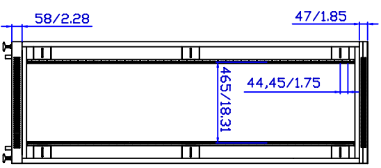
Front View with door removed
