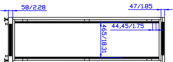
Front View with door removed
