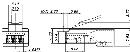
Cat6 FastPlug RJ45 Spec
